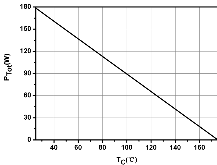
Fig.7-Power Derating
