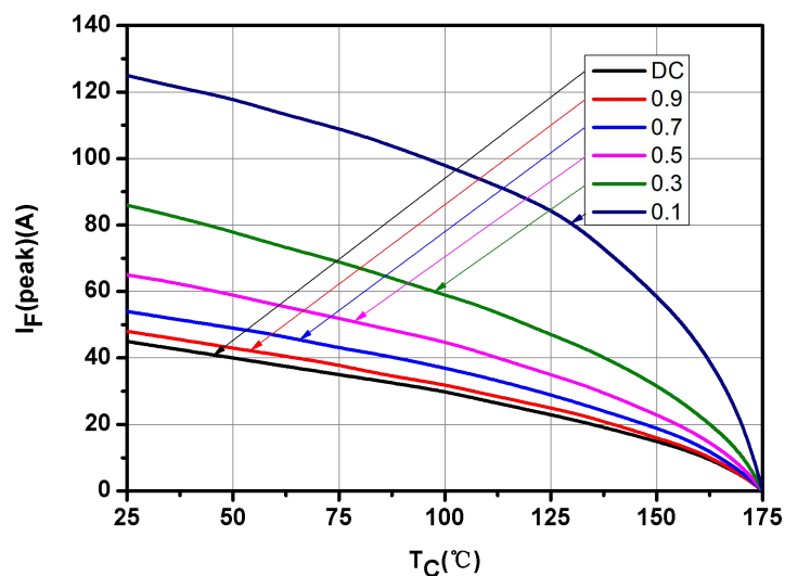
Fig.6-Current Derating
